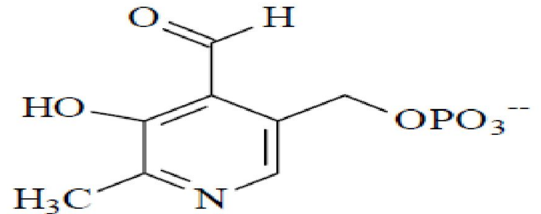
Pyridoxal Phosphate
