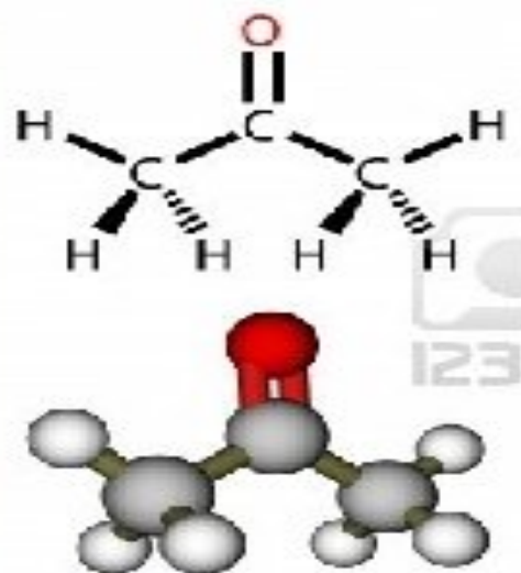
Acetone
